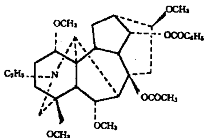
Vilmorinianine C (Forresaconitine)
