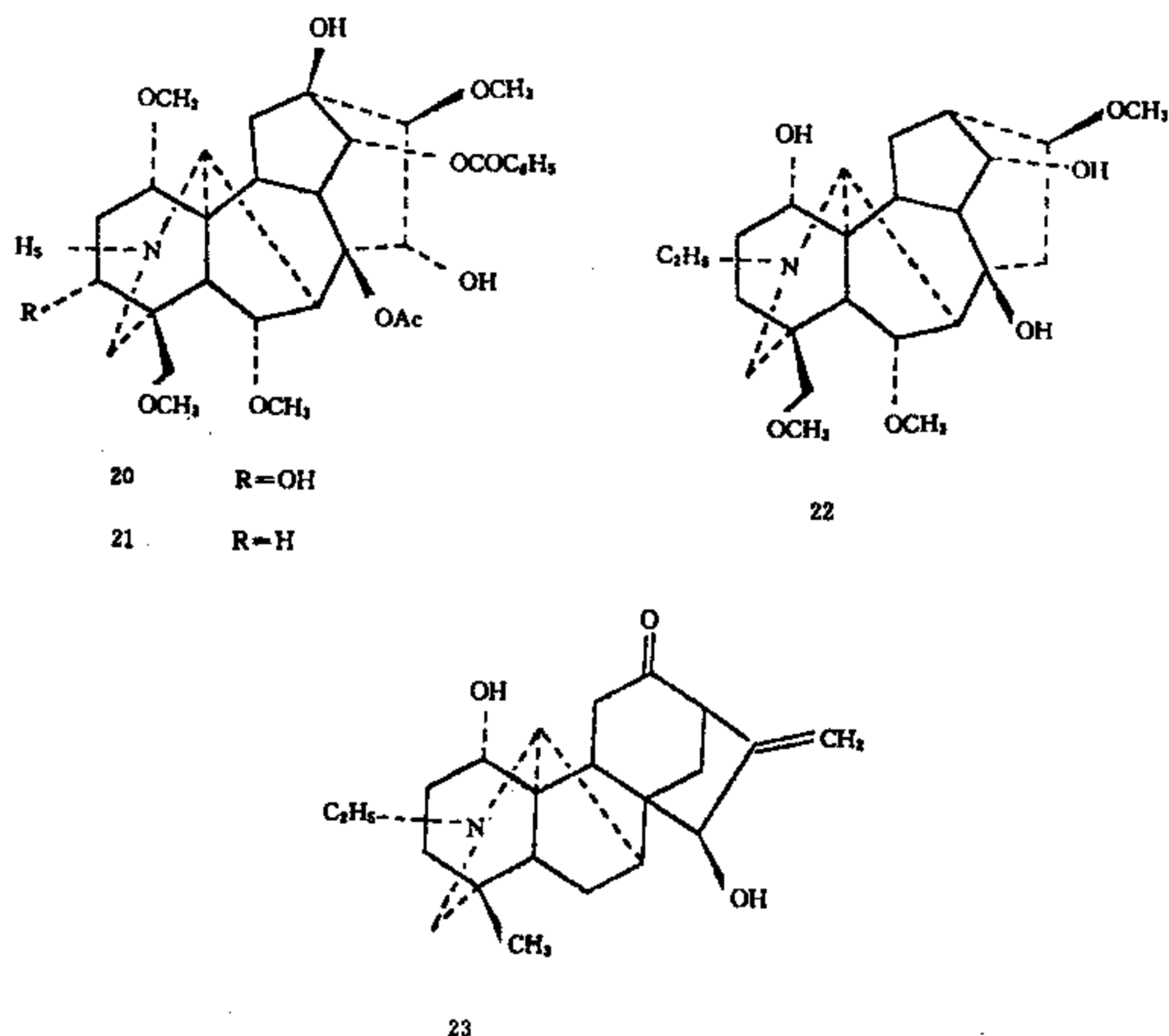
20 R=OH, aconitine 21 R=H, deoxyaconitine 22 Neoline 23 Songorine
